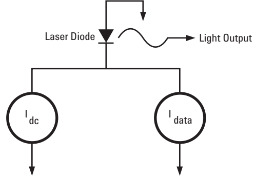
Figure 3. Direct modulated DFB laser
