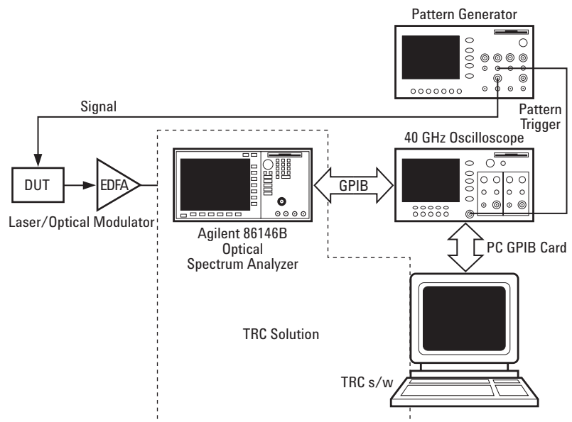
Figure 19. Block diagram TRC solution
