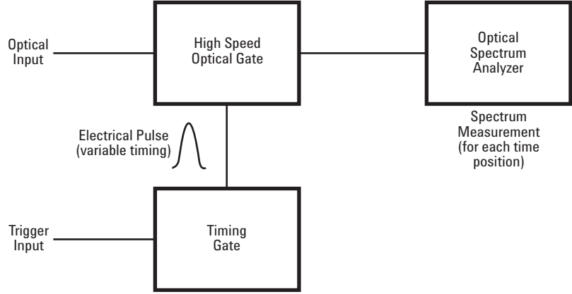
Figure 15. Optical gating + OSA
