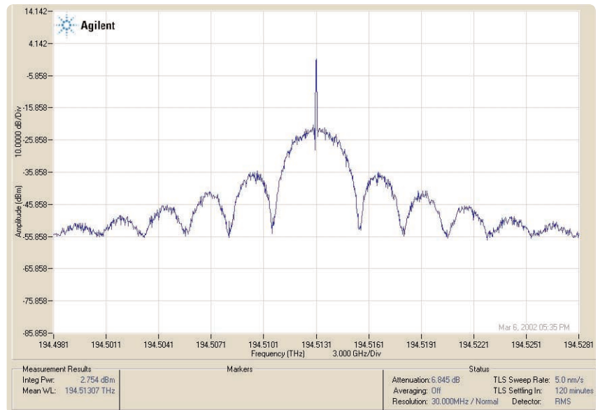
Figure 11. Mach-Zehnder Modulator Spectrum
