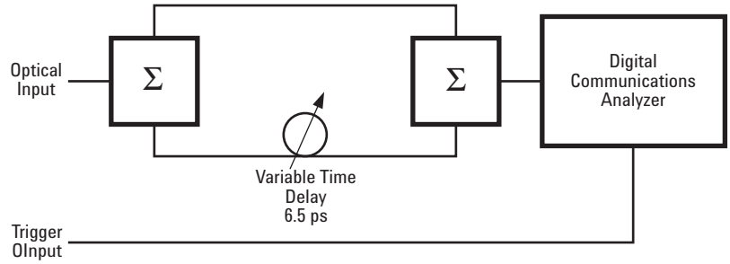
Figure 14. Mach-Zehnder Interferometer + DCA
