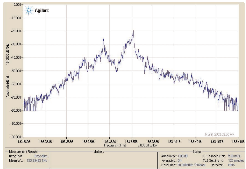
Figure 5. Agilent 83430A spectrum (using High Resolution Spectrometer)
