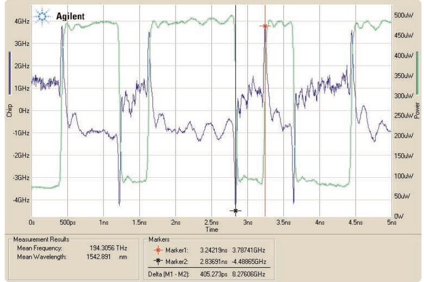
Figure 1. Time resolved chirp measurement
