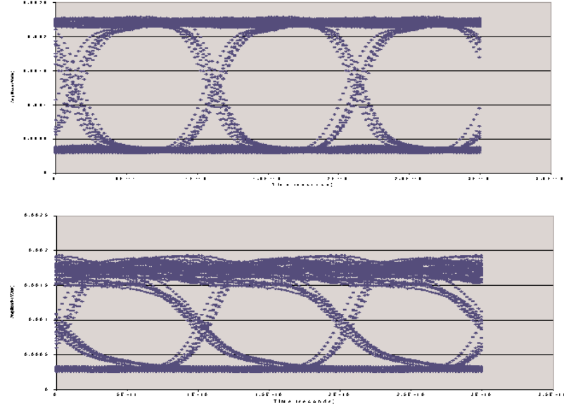
Figure 2. 10 Gb/s eye diagrams without (top) and with (bottom) the effects of chromatic dispersion.
