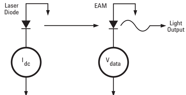
Figure 6. EML (Electro-absorption Modulated Laser)
