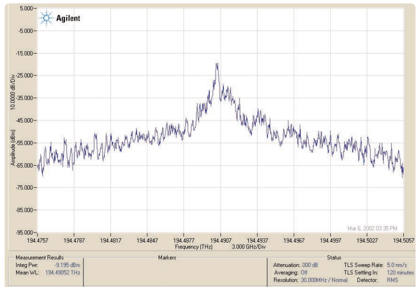
Figure 8. EML spectrum (using High Resolution Spectrometer)
