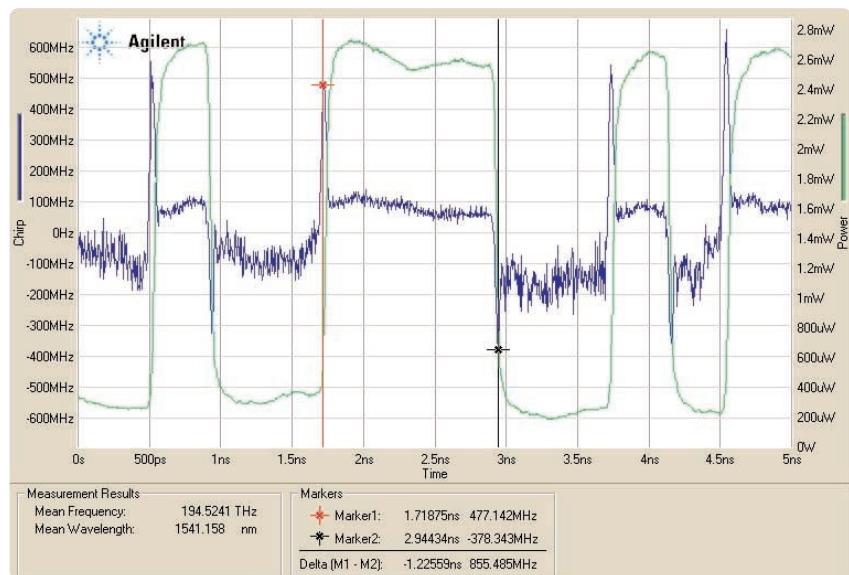
Figure 10. TRC measurement of Mach-Zehnder Modulator
