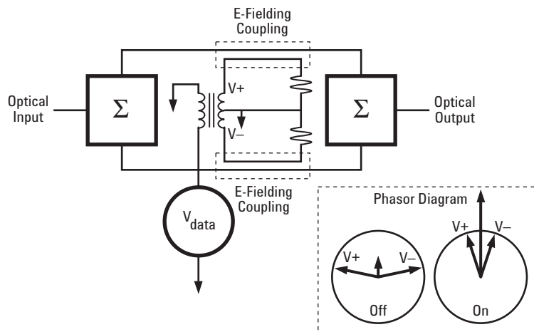
Figure 9. Mach-Zehnder Modulator
