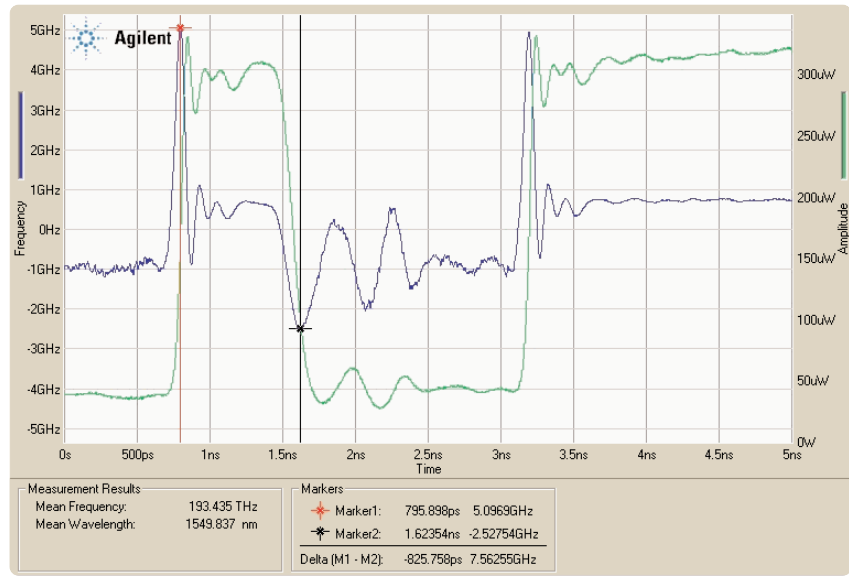
Figure 4. TRC measurement of an Agilent 83430A direct modulated DFB laser
