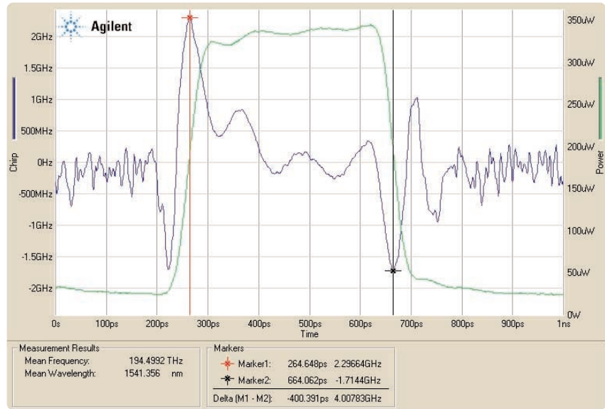
Figure 7. EML TRC
