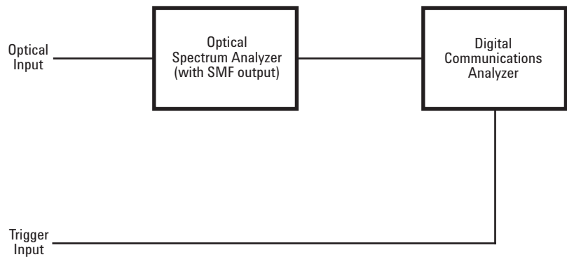
Figure 17. Monochromator + DCA
